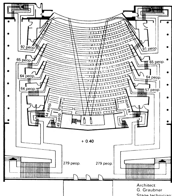
⑥ Evacuation plan: Lünen Theatre (765 seats)
